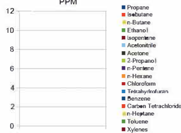
Residuals
